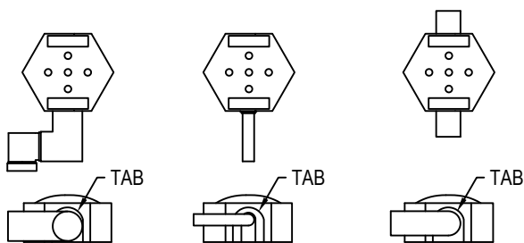
BUBBLER
